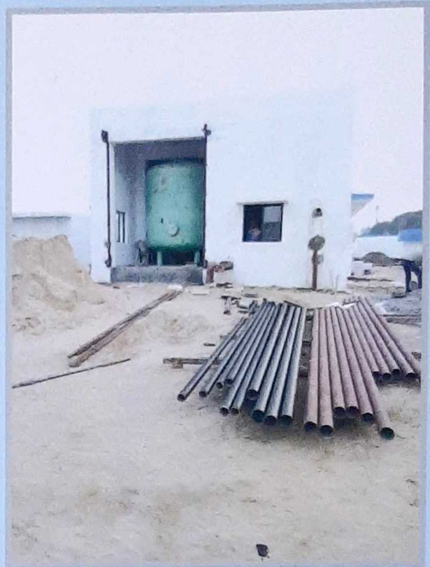
PUMP ROOM SHORT SIDE FOR 2.5 MLD SEWAGE TREATMENT PLANT CLIENT: PARADEEP PORT TRUST
